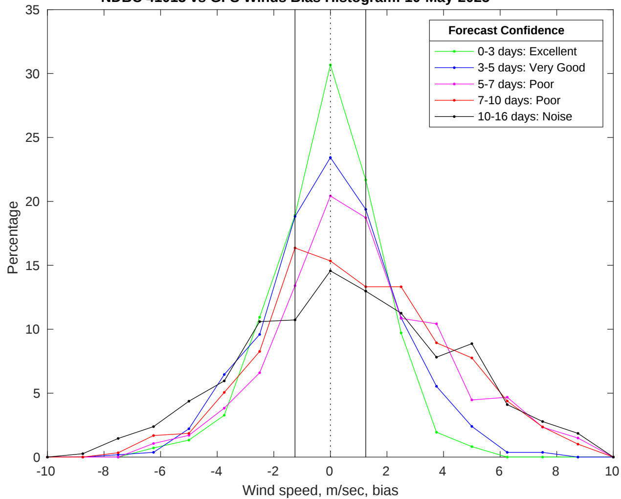
NDBC 41013 vs GFS Winds Bias Histogram: 10-May-2025
