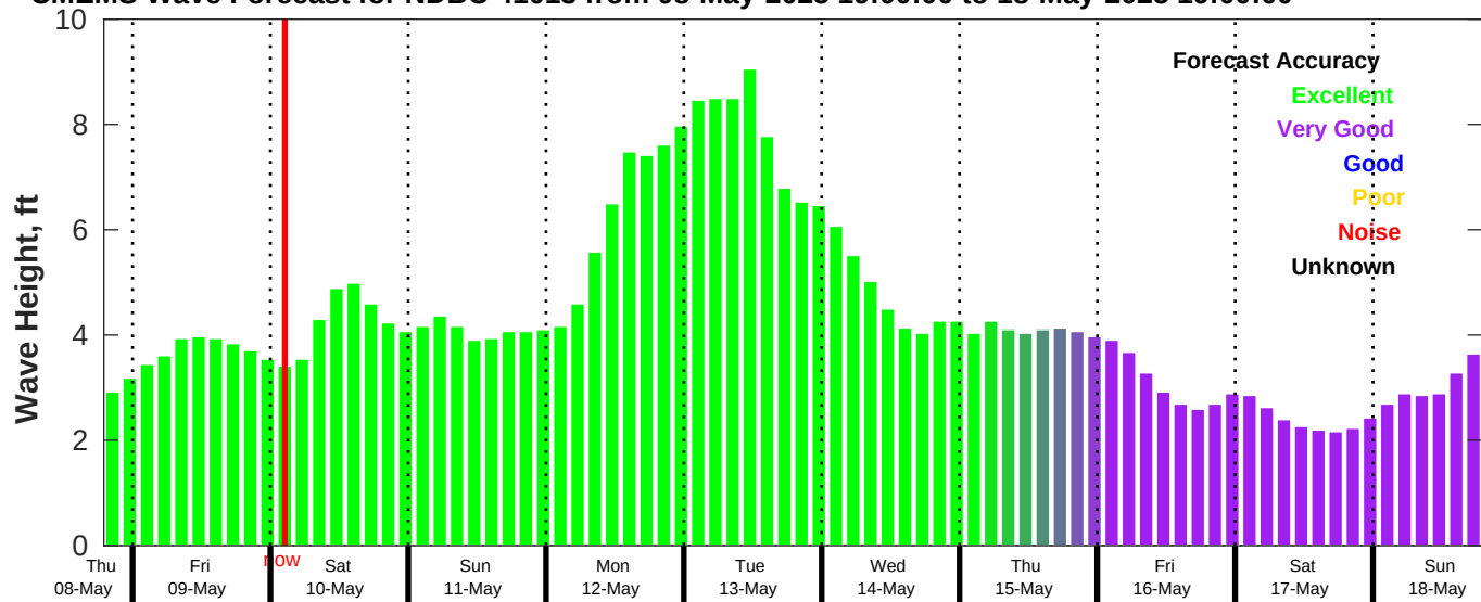
CMEMS Wave Forecast for NDBC 41013 from 08-May-2025 19:00:00 to 18-May-2025 19:00:00
