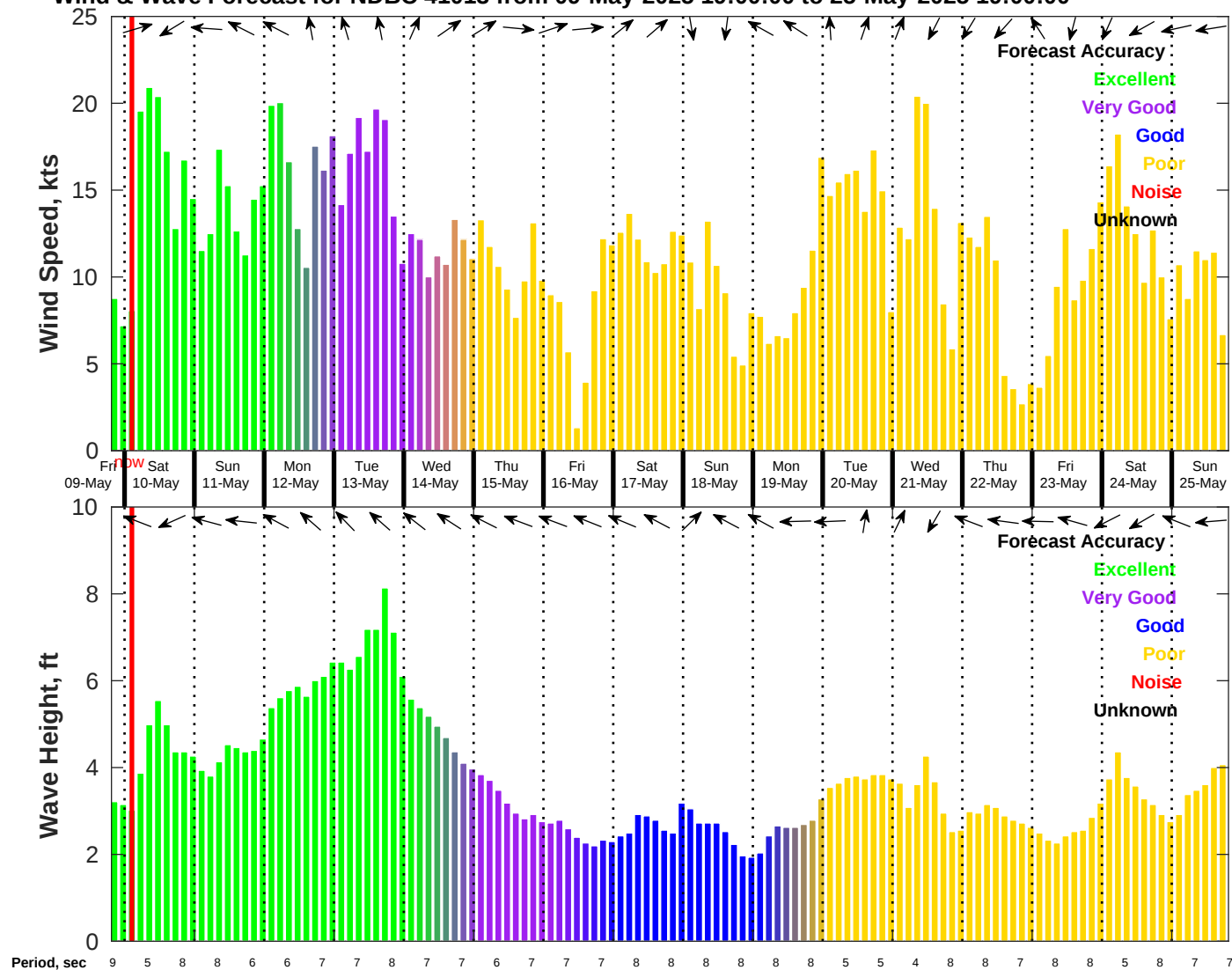
Wind & Wave Forecast for NDBC 41013 from 09-May-2025 19:00:00 to 25-May-2025 19:00:00
