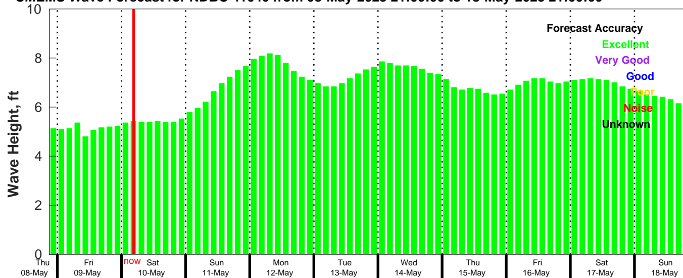
CMEMS Wave Forecast for NDBC 41040 from 08-May-2025 21:00:00 to 18-May-2025 21:00:00
