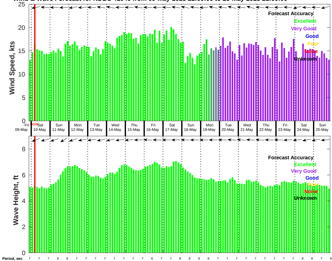
Wind & Wave Forecast for NDBC 41040 from 09-May-2025 21:00:00 to 25-May-2025 21:00:00
