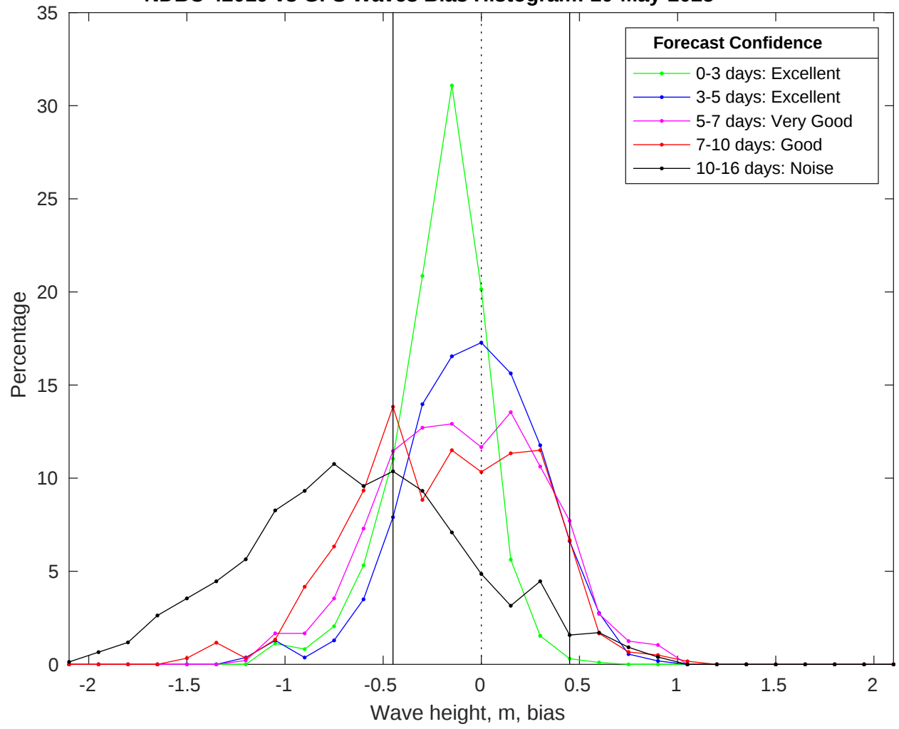
NDBC 42019 vs GFS Waves Bias Histogram: 10-May-2025
