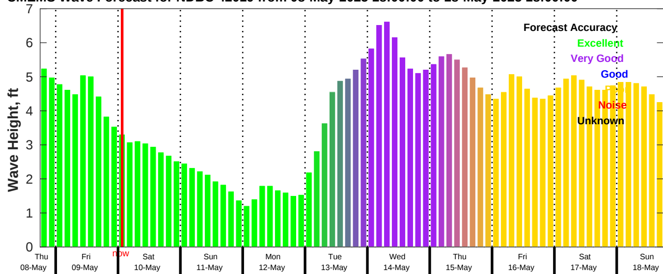
CMEMS Wave Forecast for NDBC 42019 from 08-May-2025 18:00:00 to 18-May-2025 18:00:00
