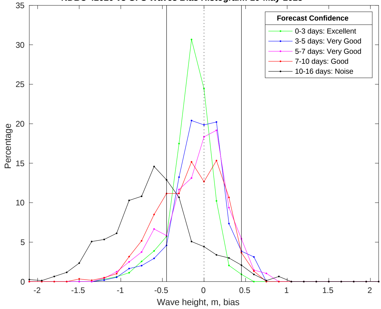
NDBC 42020 vs GFS Waves Bias Histogram: 10-May-2025
