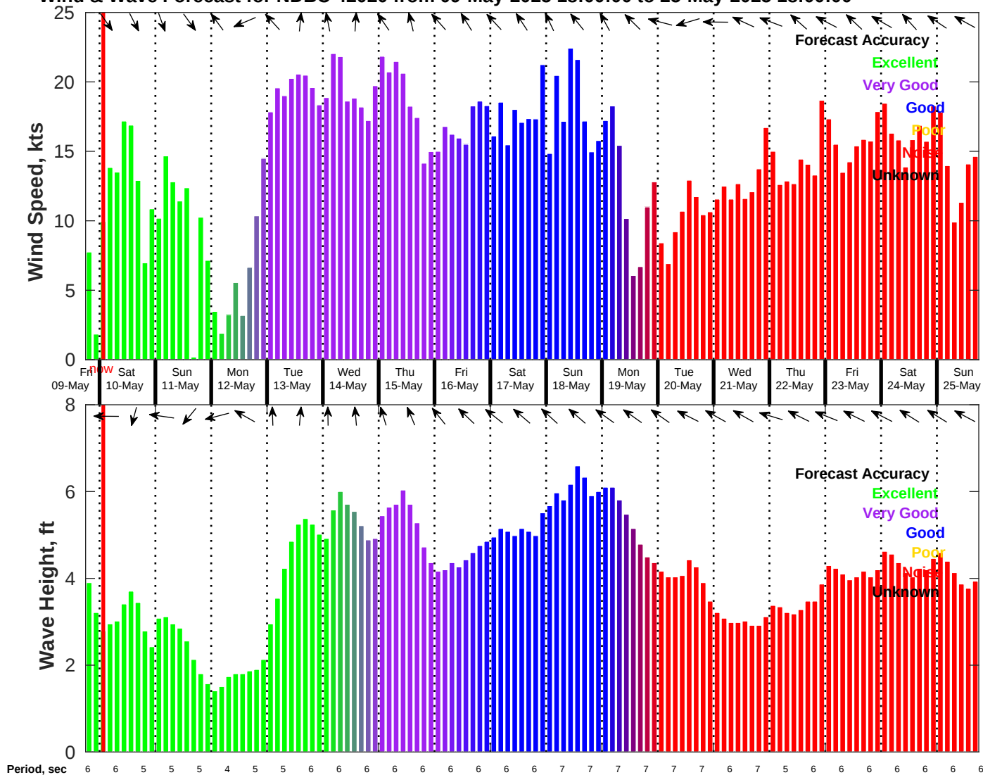
Wind & Wave Forecast for NDBC 42020 from 09-May-2025 18:00:00 to 25-May-2025 18:00:00
