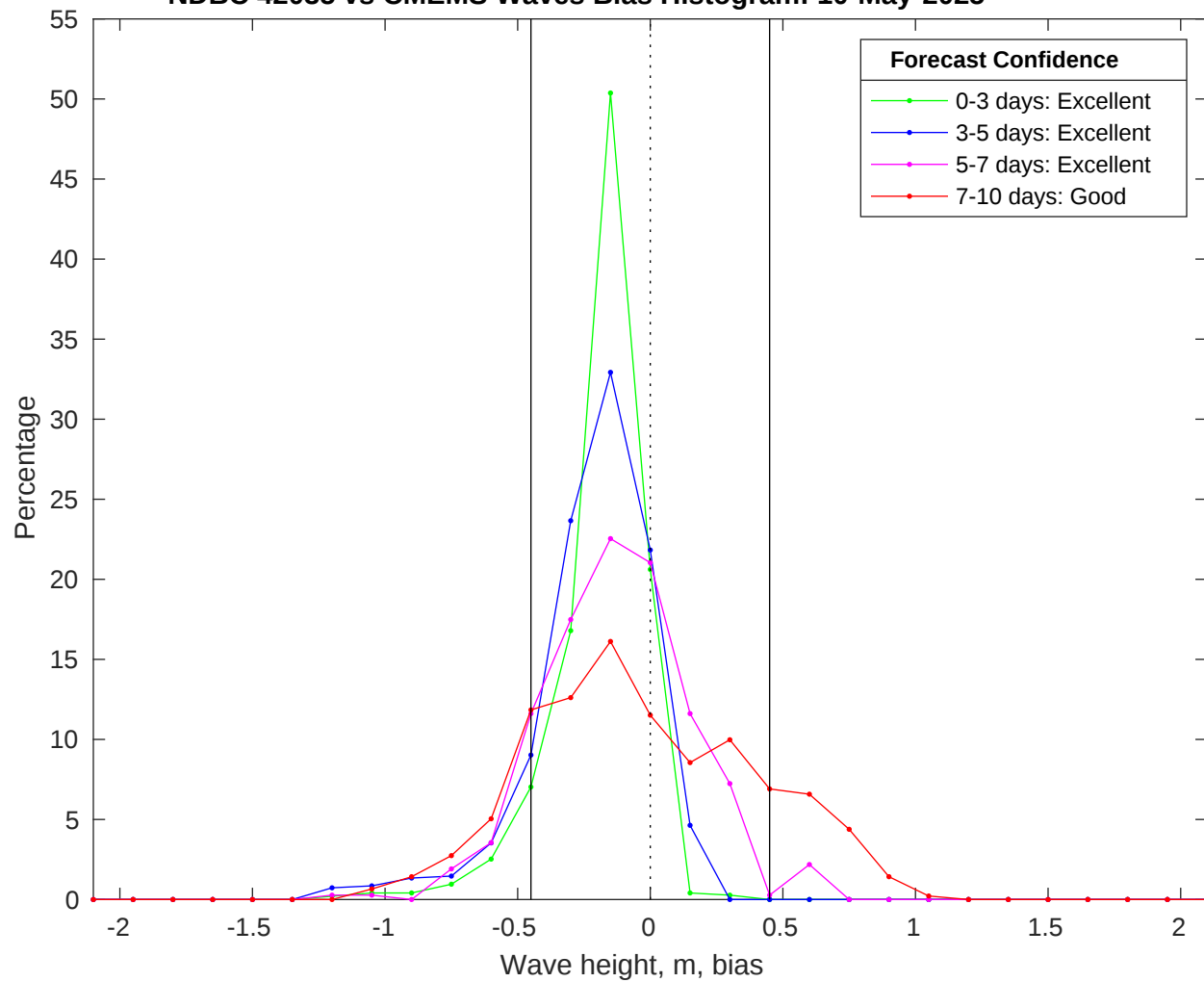
NDBC 42035 vs CMEMS Waves Bias Histogram: 10-May-2025
