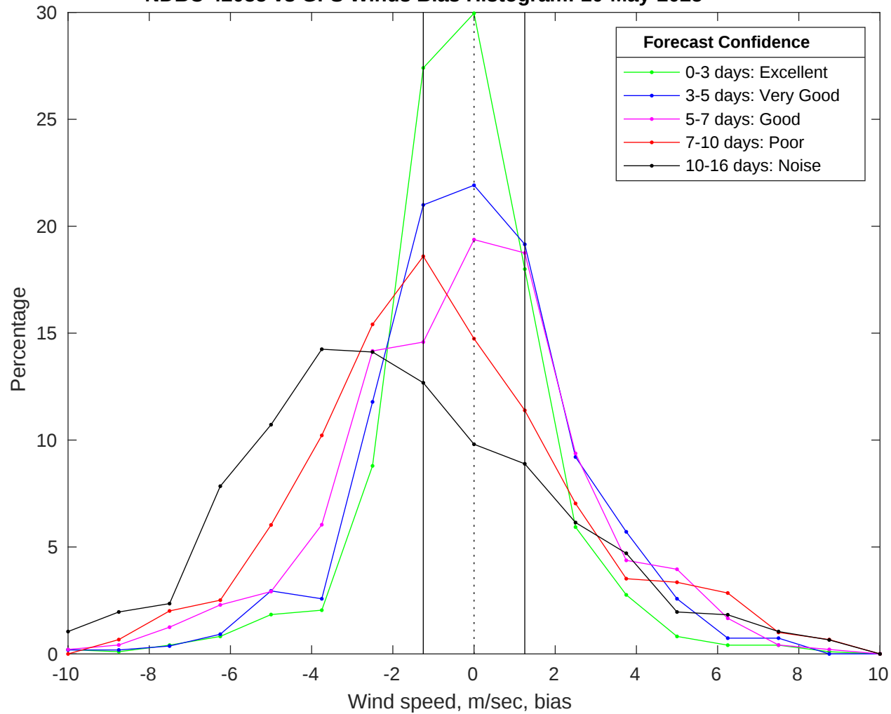
NDBC 42035 vs GFS Winds Bias Histogram: 10-May-2025
