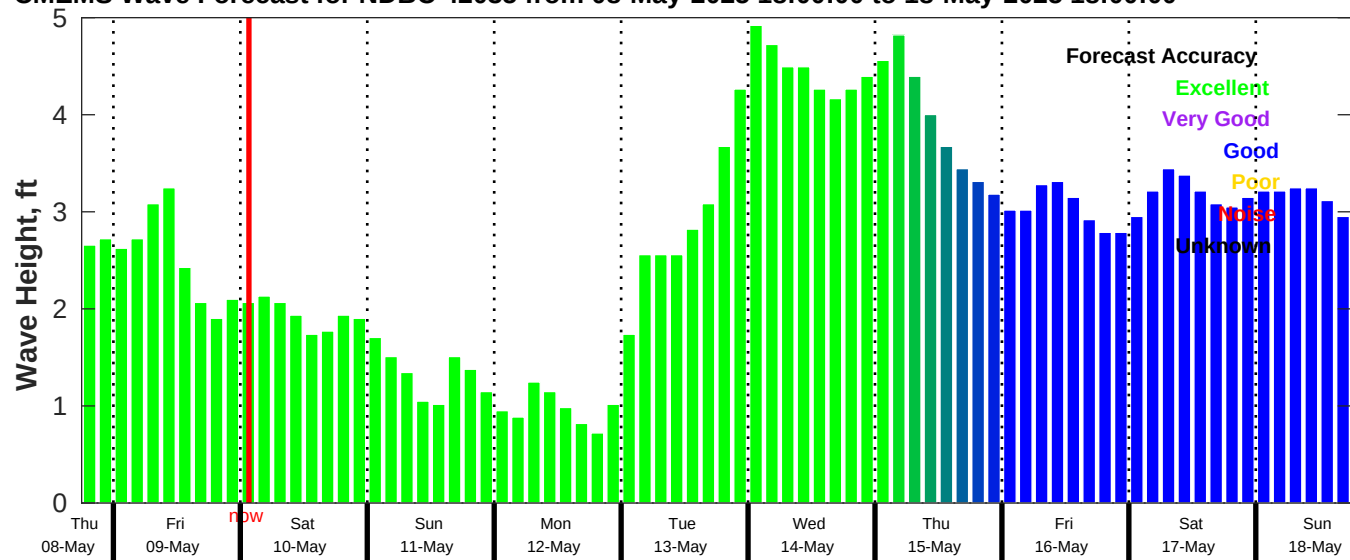
CMEMS Wave Forecast for NDBC 42035 from 08-May-2025 18:00:00 to 18-May-2025 18:00:00
