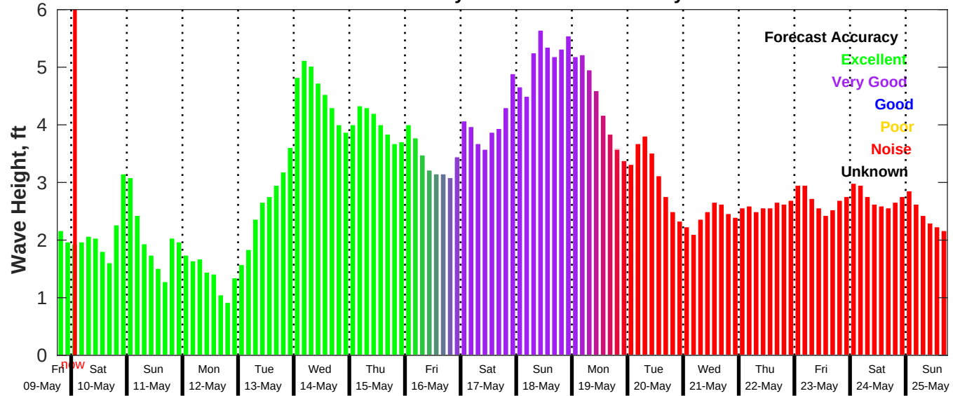
GFS Wave Forecast for NDBC 42035 from 09-May-2025 18:00:00 to 25-May-2025 18:00:00
