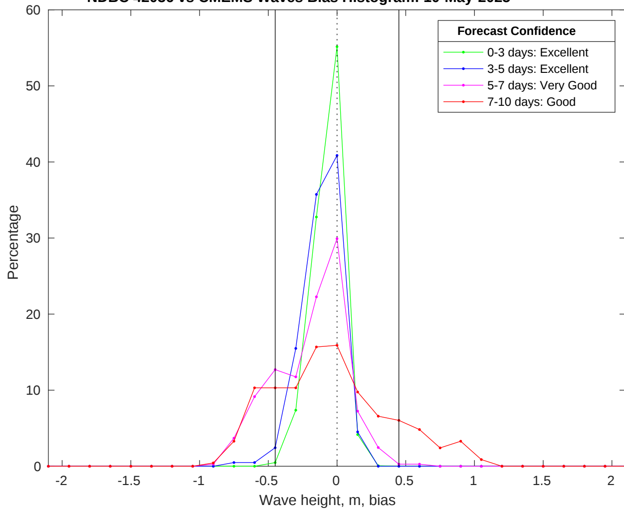
NDBC 42036 vs CMEMS Waves Bias Histogram: 10-May-2025
