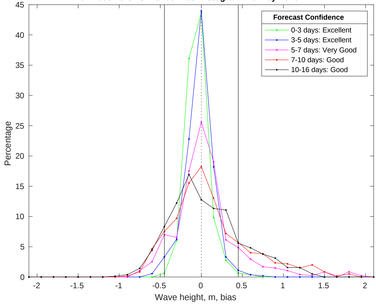
NDBC 42036 vs GFS Waves Bias Histogram: 10-May-2025
