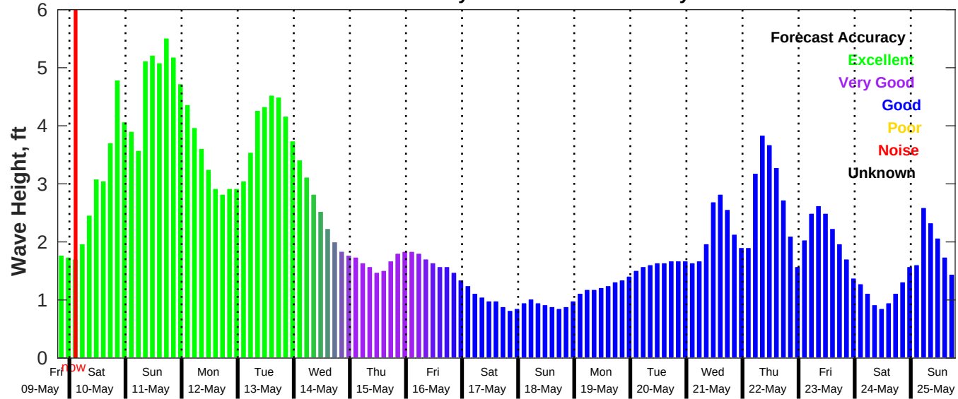
GFS Wave Forecast for NDBC 42036 from 09-May-2025 19:00:00 to 25-May-2025 19:00:00
