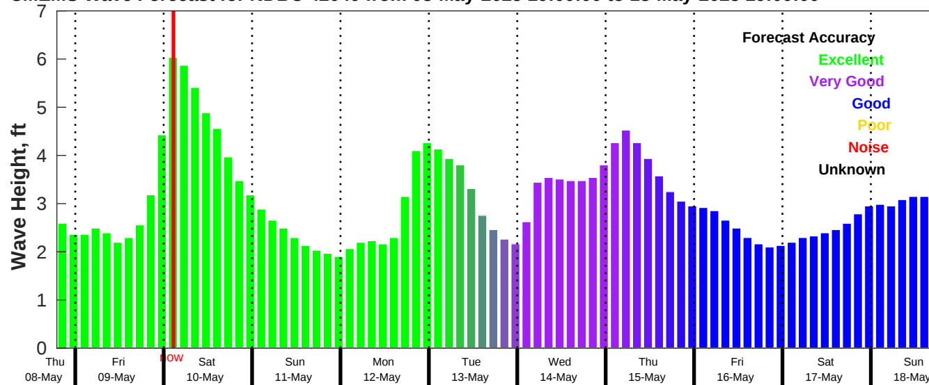
CMEMS Wave Forecast for NDBC 42040 from 08-May-2025 19:00:00 to 18-May-2025 19:00:00
