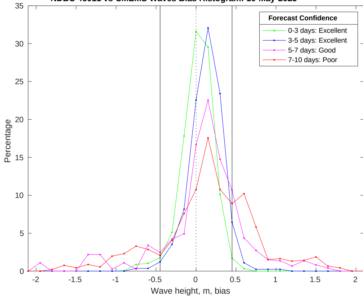
NDBC 46011 vs CMEMS Waves Bias Histogram: 10-May-2025
