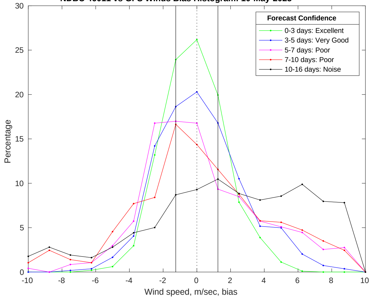
NDBC 46011 vs GFS Winds Bias Histogram: 10-May-2025
