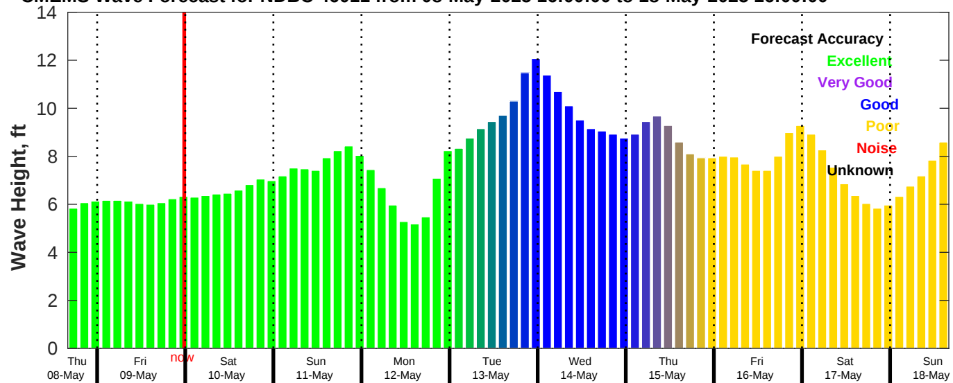
CMEMS Wave Forecast for NDBC 46011 from 08-May-2025 16:00:00 to 18-May-2025 16:00:00
