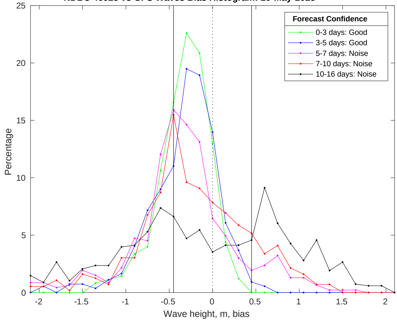
NDBC 46028 vs GFS Waves Bias Histogram: 10-May-2025
