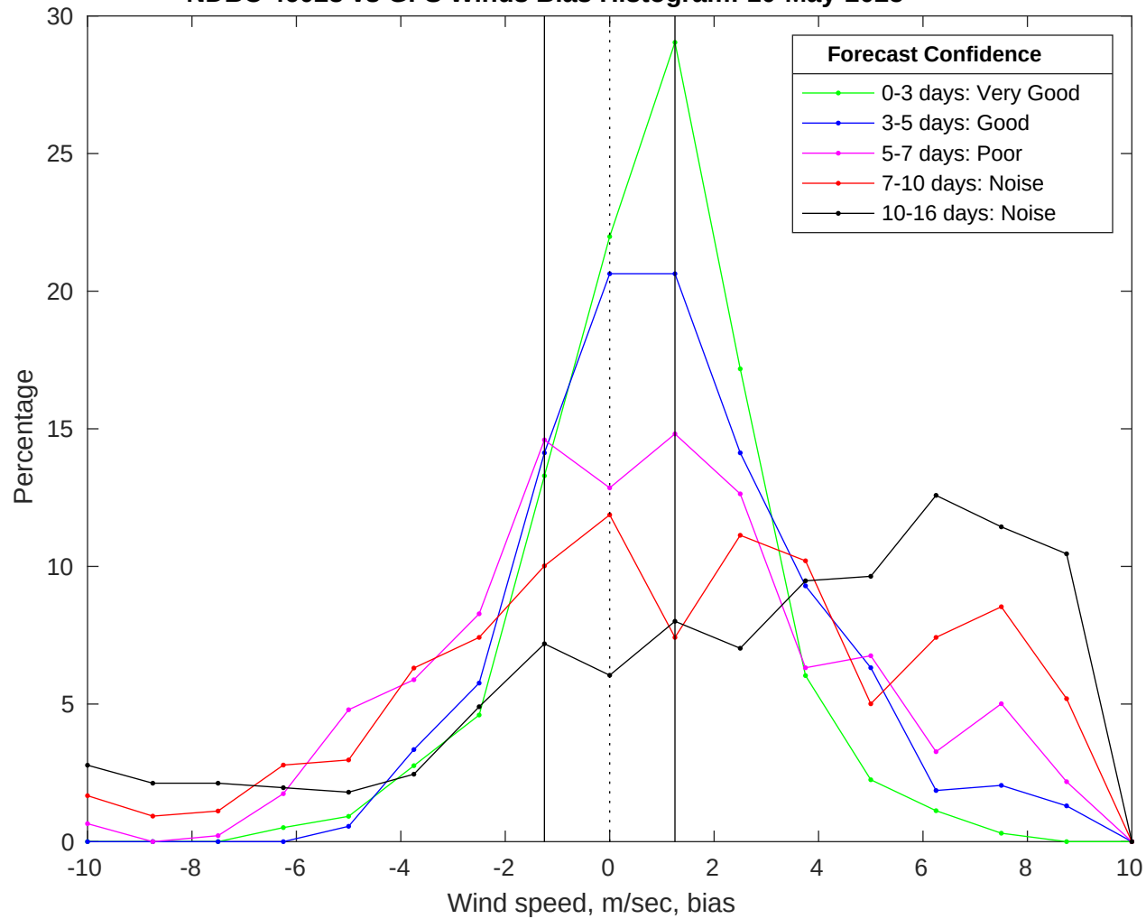
NDBC 46028 vs GFS Winds Bias Histogram: 10-May-2025
