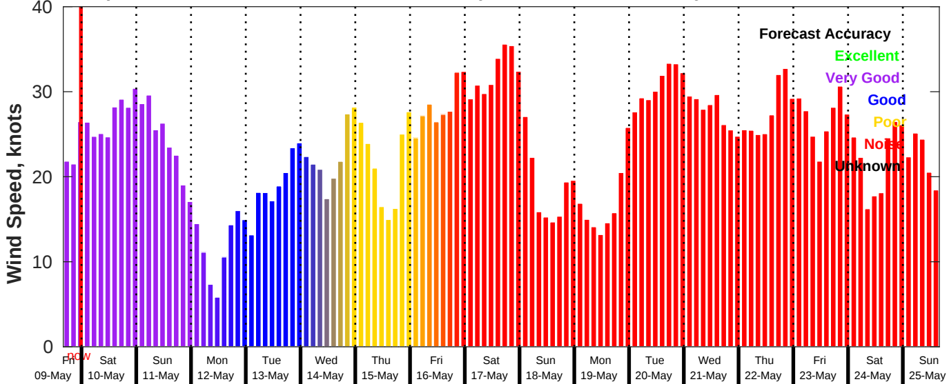
GFS Wind Speed Forecast for NDBC 46028 from 09-May-2025 16:00:00 to 25-May-2025 16:00:00
