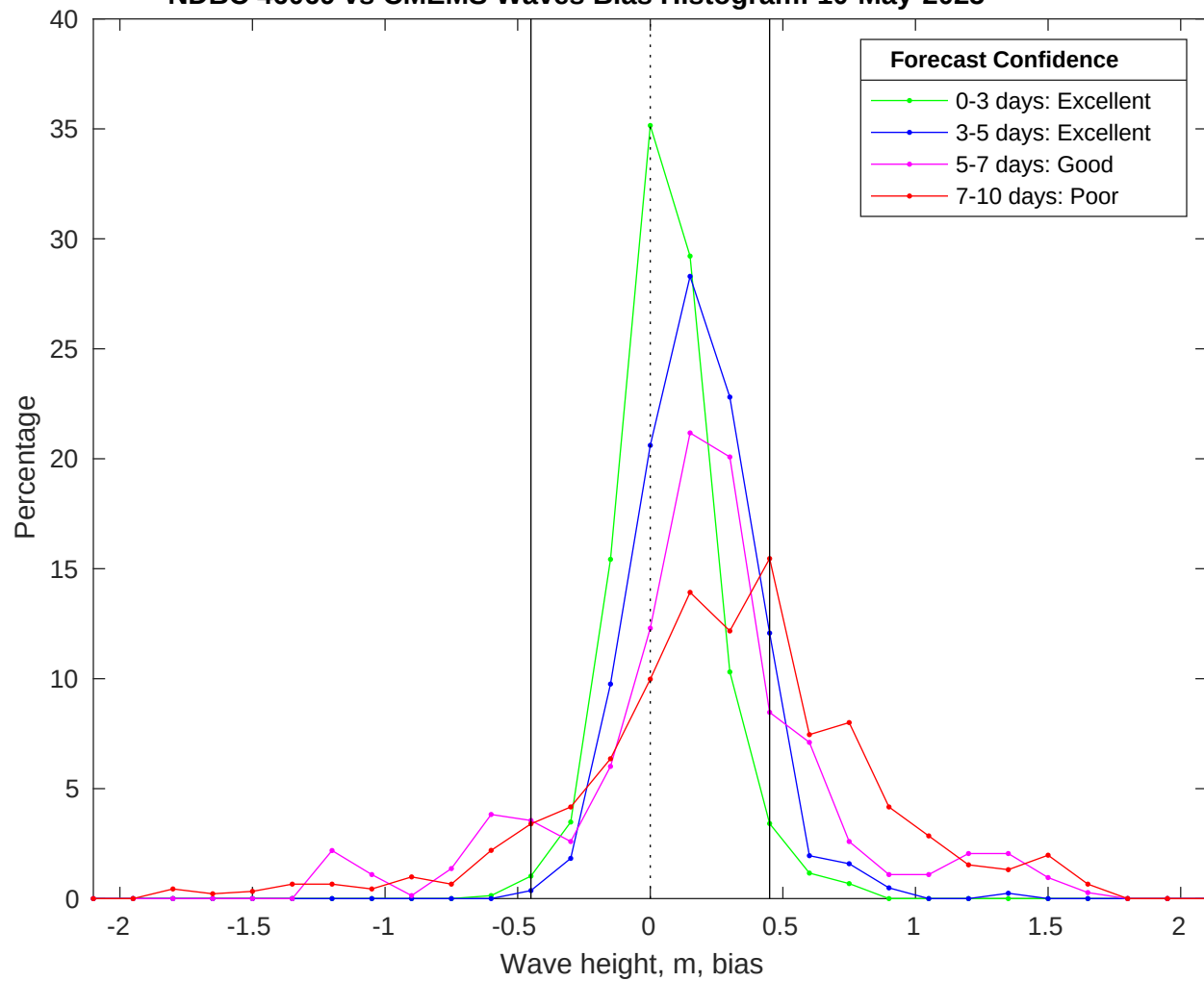
NDBC 46069 vs CMEMS Waves Bias Histogram: 10-May-2025
