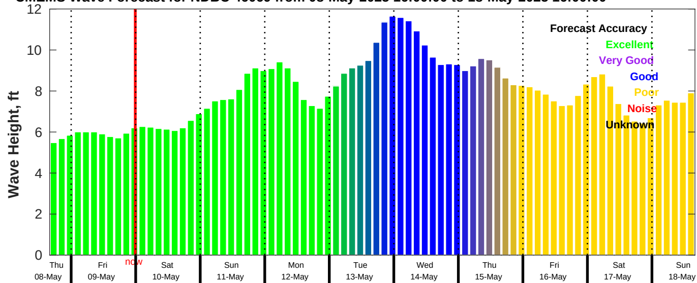
CMEMS Wave Forecast for NDBC 46069 from 08-May-2025 16:00:00 to 18-May-2025 16:00:00
