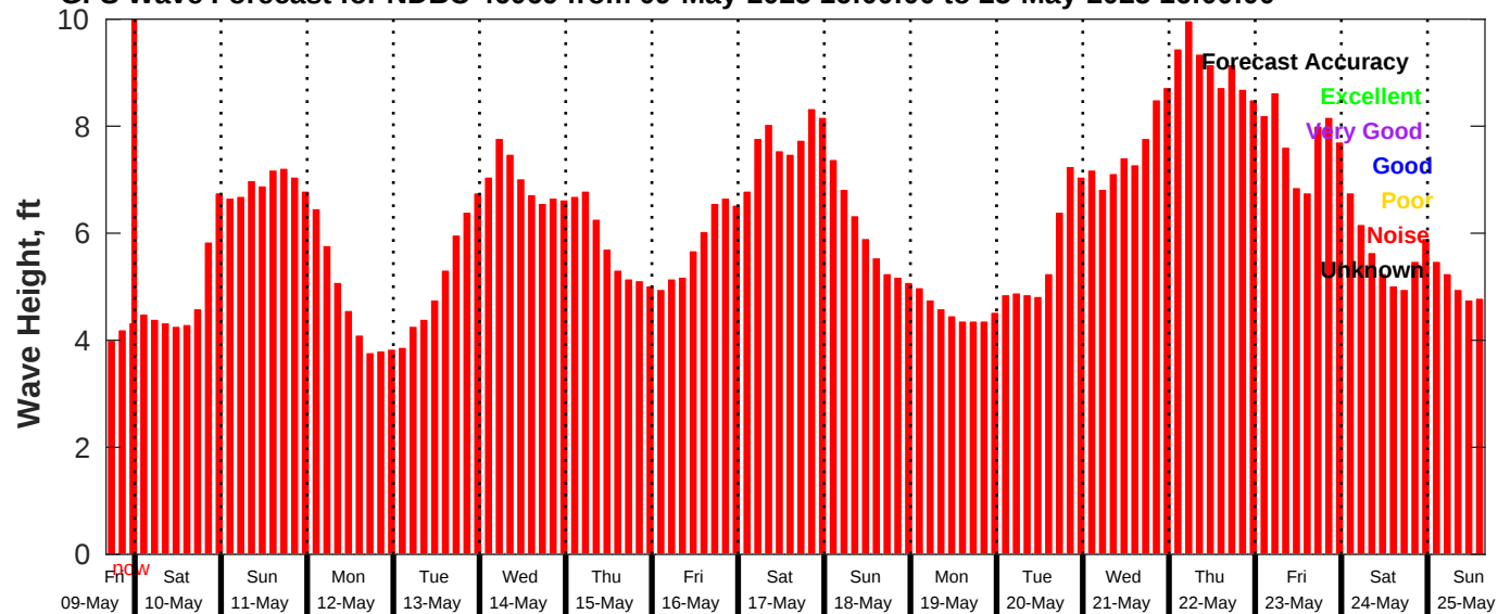
GFS Wave Forecast for NDBC 46069 from 09-May-2025 16:00:00 to 25-May-2025 16:00:00
