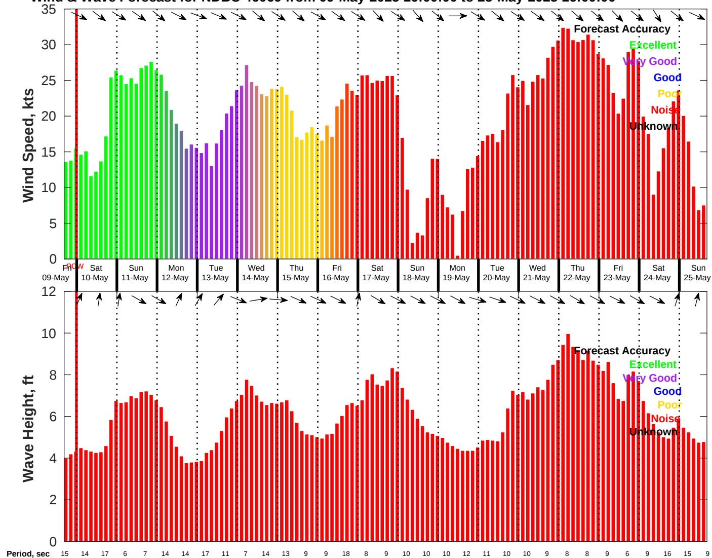
Wind & Wave Forecast for NDBC 46069 from 09-May-2025 16:00:00 to 25-May-2025 16:00:00
