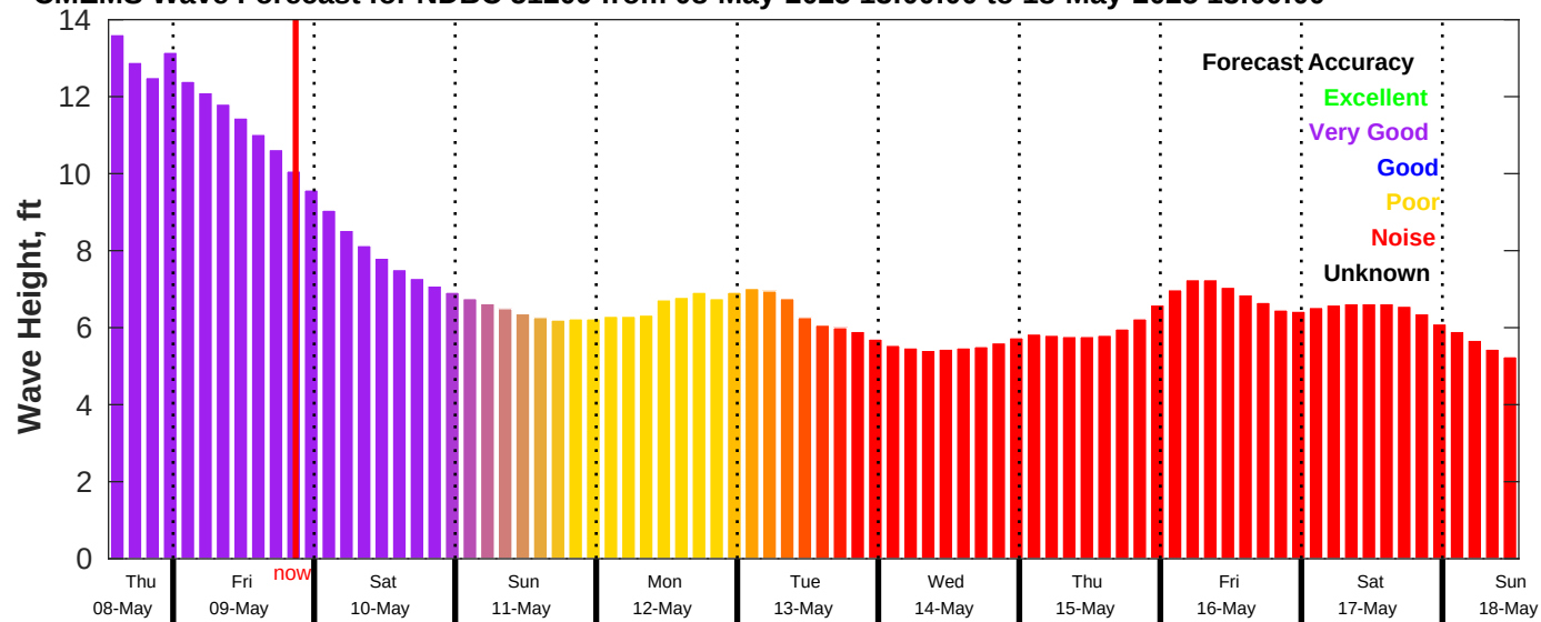
CMEMS Wave Forecast for NDBC 51209 from 08-May-2025 13:00:00 to 18-May-2025 13:00:00
