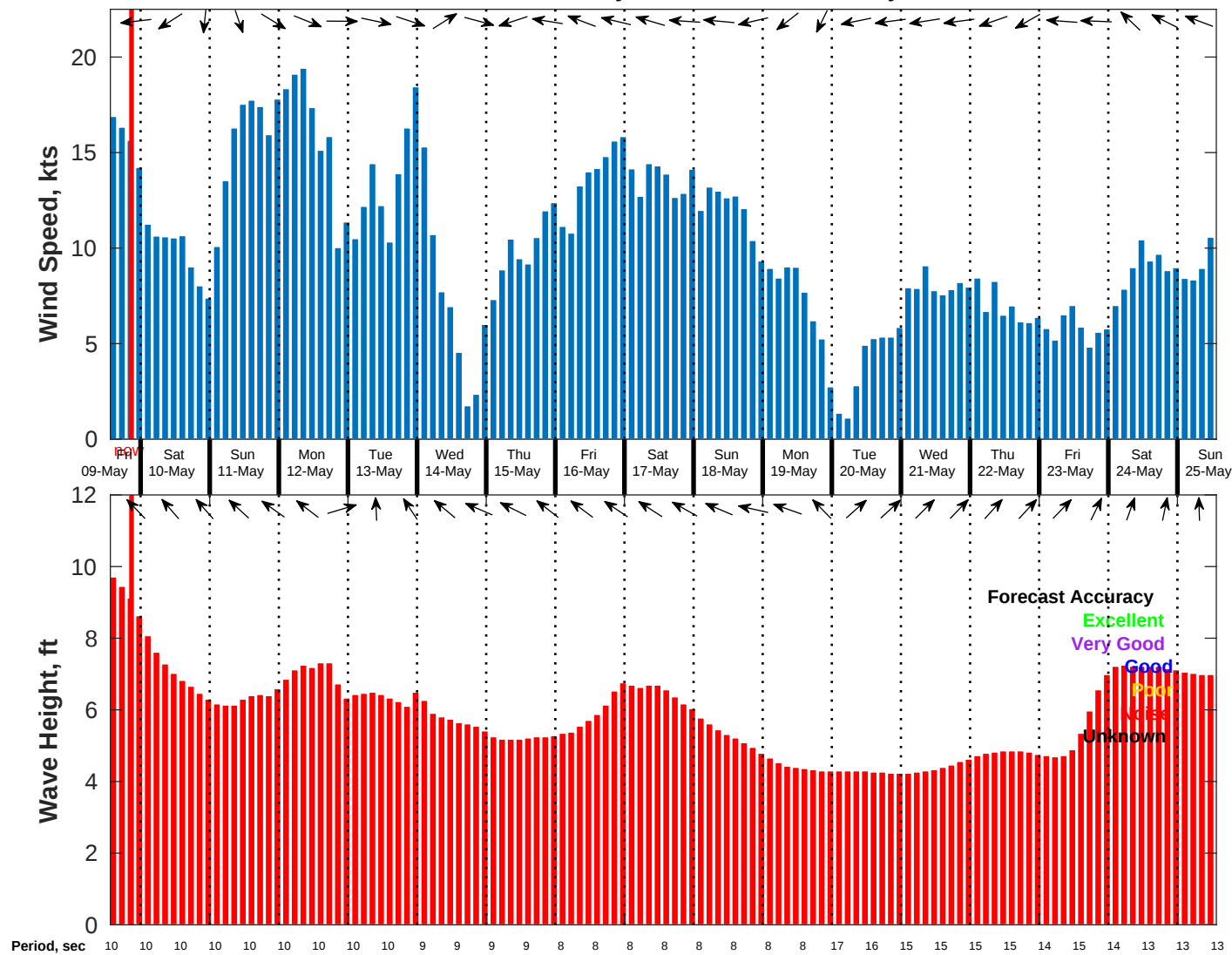
Wind & Wave Forecast for NDBC 51209 from 09-May-2025 13:00:00 to 25-May-2025 13:00:00
