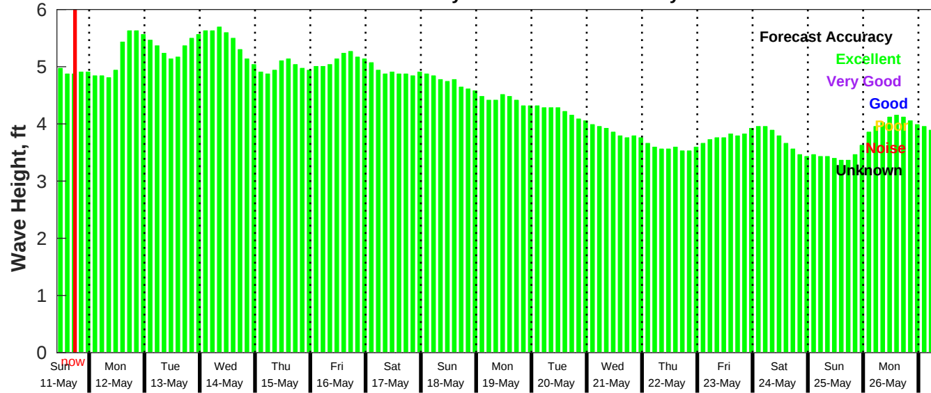
GFS Wave Forecast for NDBC 52211 from 10-May-2025 10:00:00 to 26-May-2025 10:00:00
