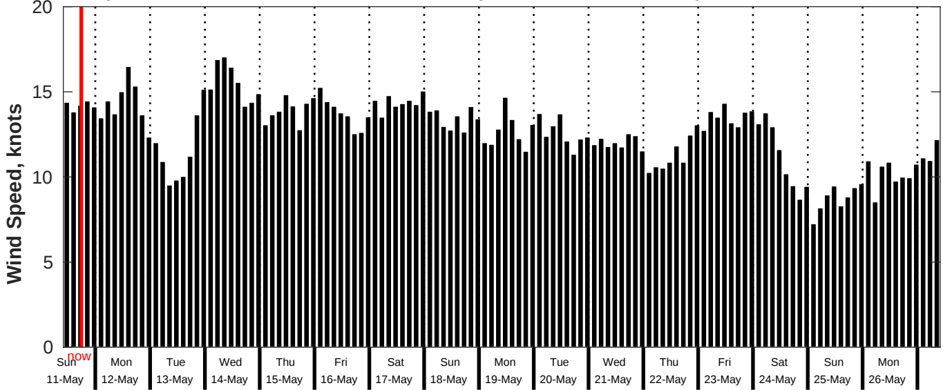
GFS Wind Speed Forecast for NDBC 52211 from 10-May-2025 10:00:00 to 26-May-2025 10:00:00
