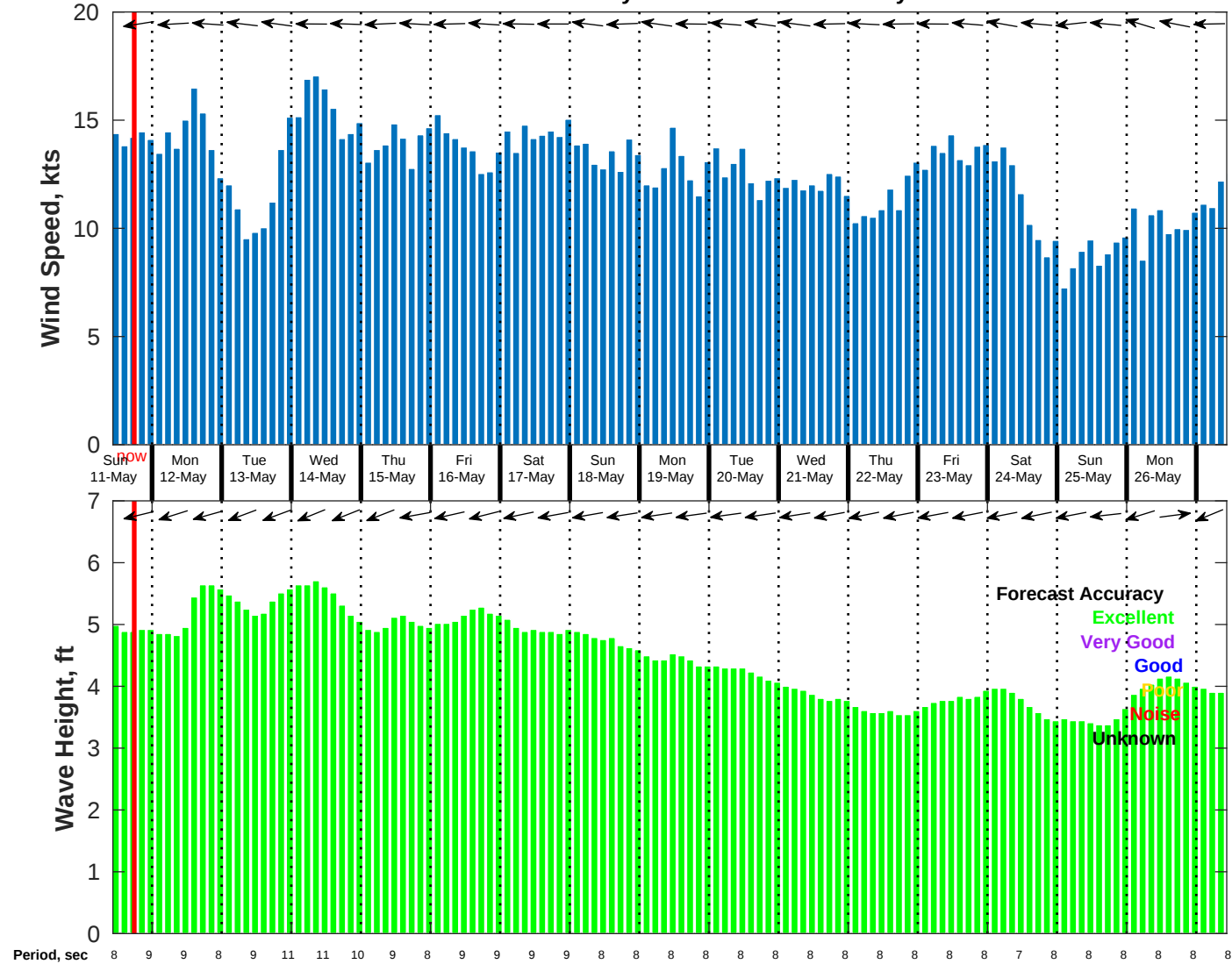
Wind & Wave Forecast for NDBC 52211 from 10-May-2025 10:00:00 to 26-May-2025 10:00:00
