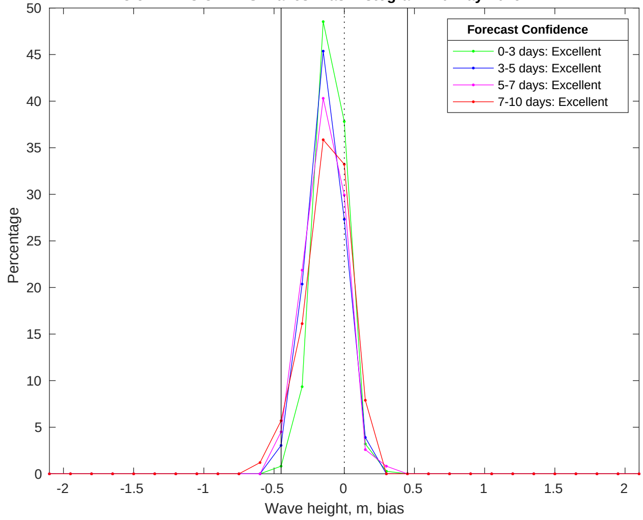
NDBC 52212 vs CMEMS Waves Bias Histogram: 10-May-2025
