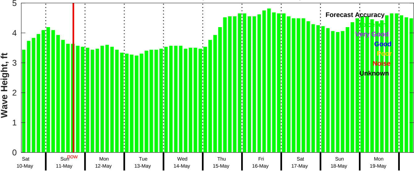
CMEMS Wave Forecast for NDBC 52212 from 09-May-2025 09:00:00 to 19-May-2025 09:00:00
