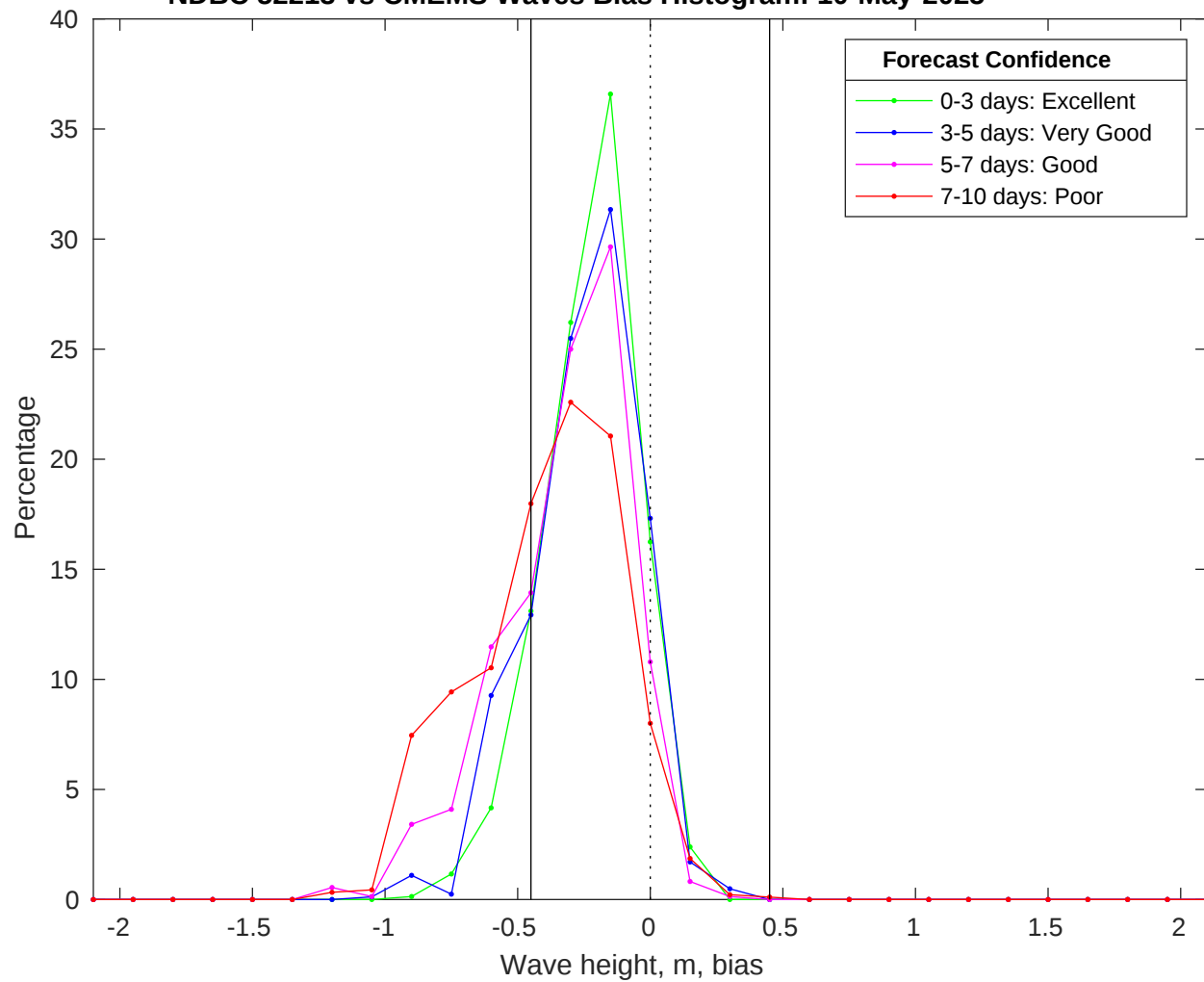
NDBC 52213 vs CMEMS Waves Bias Histogram: 10-May-2025
