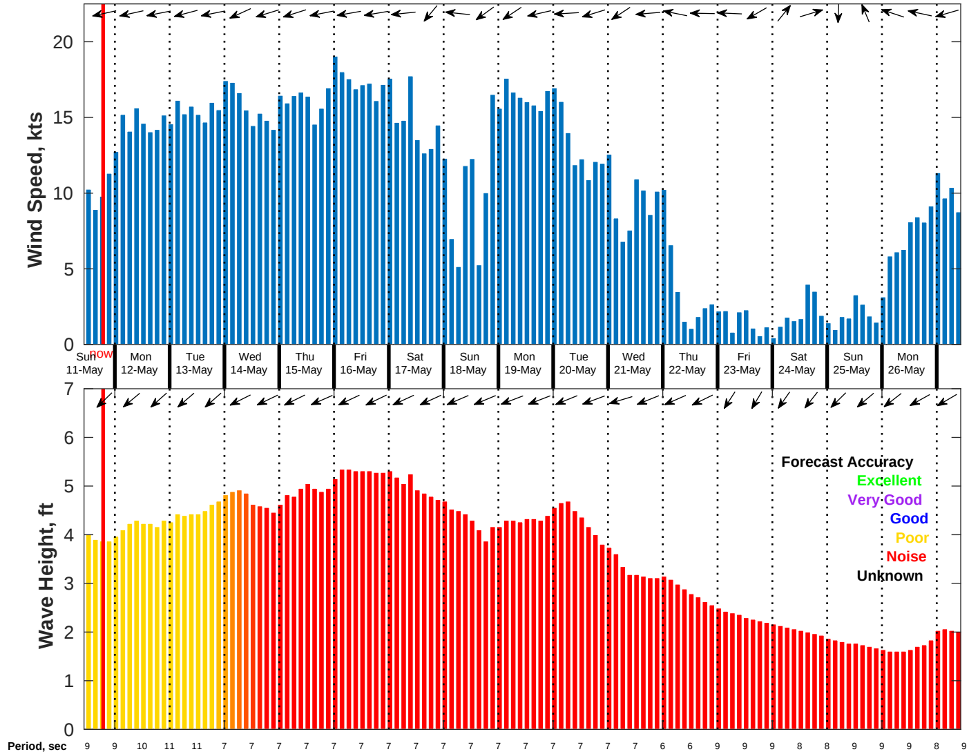
Wind & Wave Forecast for NDBC 52213 from 10-May-2025 11:00:00 to 26-May-2025 11:00:00
