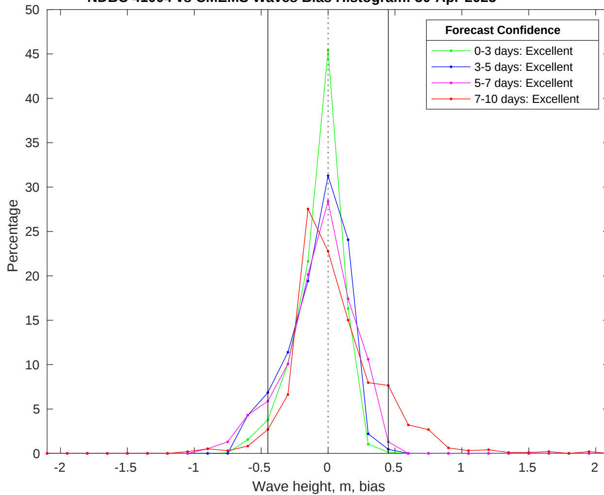
NDBC 41004 vs CMEMS Waves Bias Histogram: 30-Apr-2025
