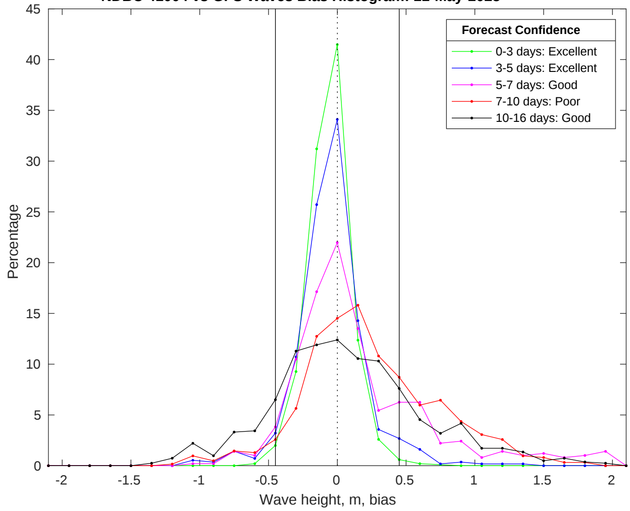
NDBC 41004 vs GFS Waves Bias Histogram: 11-May-2025
