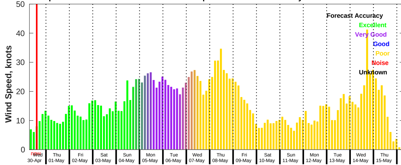
GFS Wind Speed Forecast for NDBC 41004 from 30-Apr-2025 07:00:00 to 16-May-2025 07:00:00
