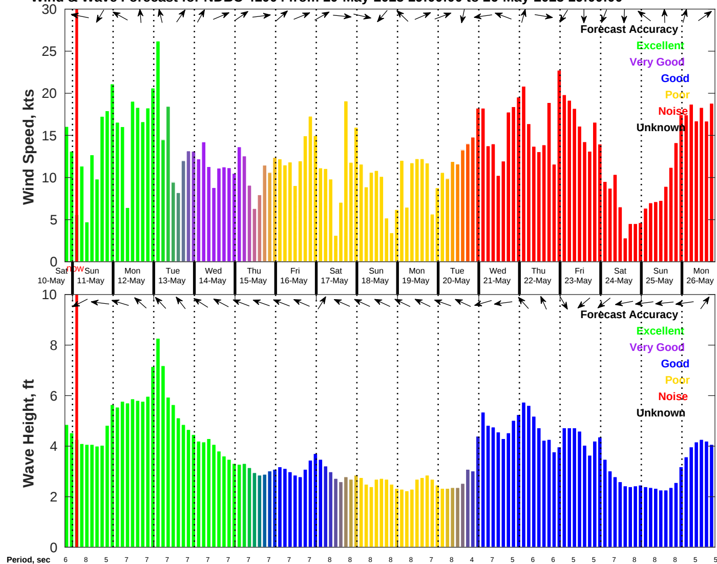
Wind & Wave Forecast for NDBC 41004 from 10-May-2025 19:00:00 to 26-May-2025 19:00:00
