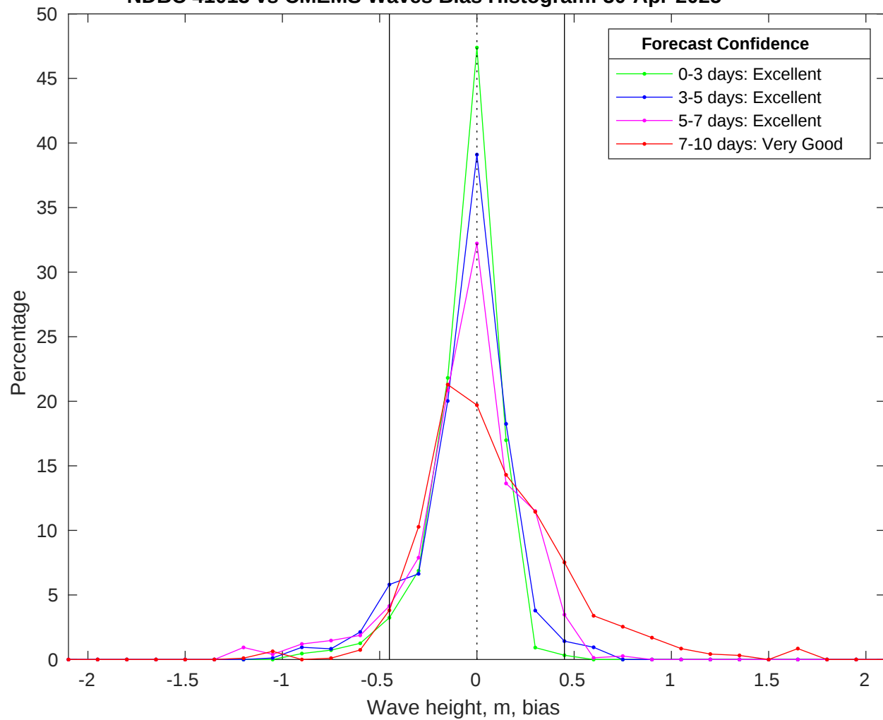
NDBC 41013 vs CMEMS Waves Bias Histogram: 30-Apr-2025
