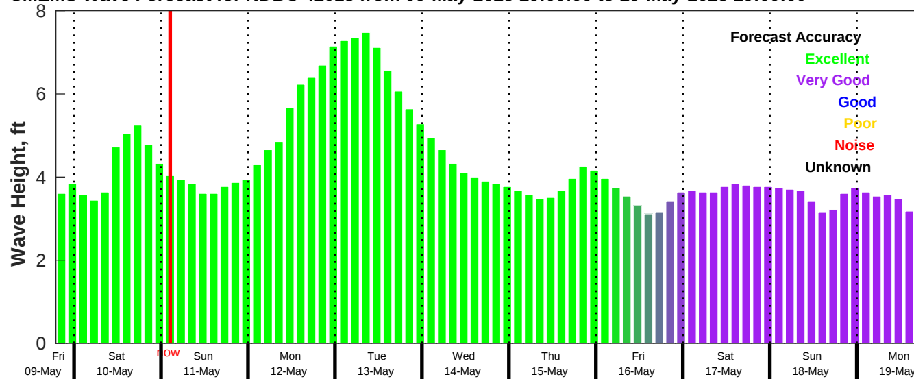
CMEMS Wave Forecast for NDBC 41013 from 09-May-2025 19:00:00 to 19-May-2025 19:00:00
