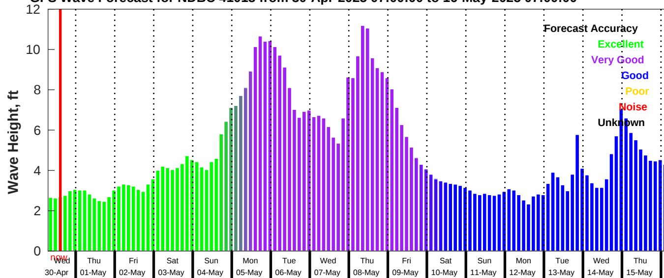
GFS Wave Forecast for NDBC 41013 from 30-Apr-2025 07:00:00 to 16-May-2025 07:00:00
