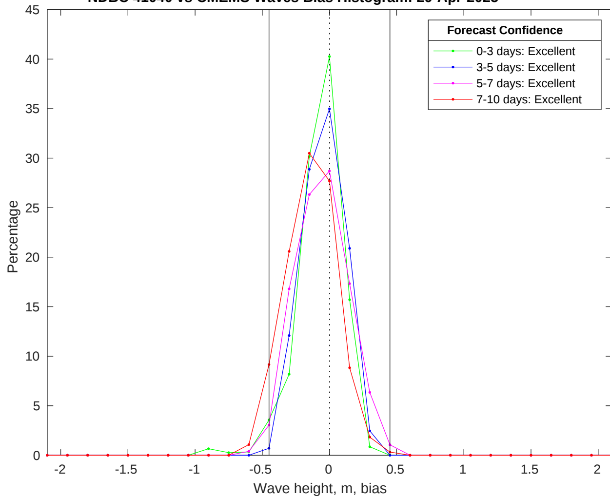
NDBC 41040 vs CMEMS Waves Bias Histogram: 29-Apr-2025
