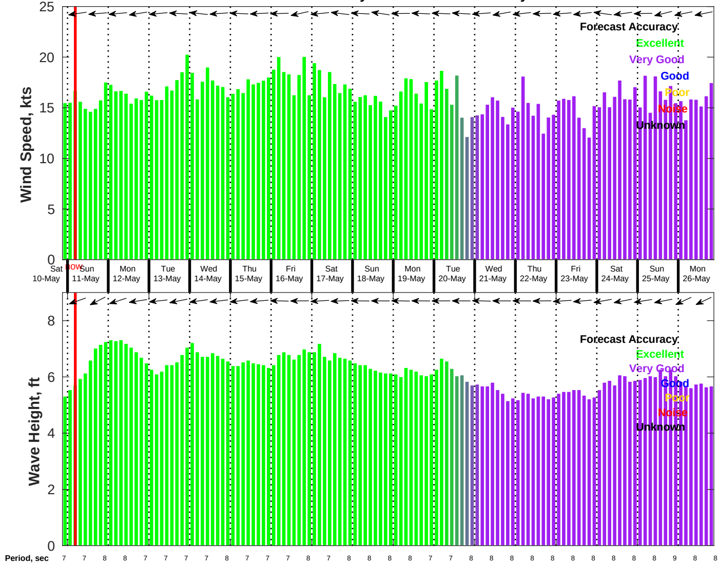
Wind & Wave Forecast for NDBC 41040 from 10-May-2025 21:00:00 to 26-May-2025 21:00:00
