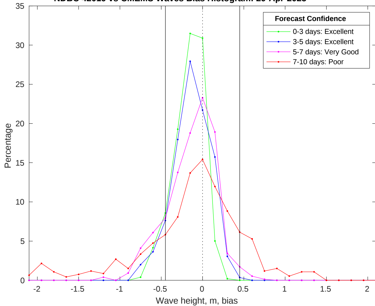
NDBC 42019 vs CMEMS Waves Bias Histogram: 29-Apr-2025
