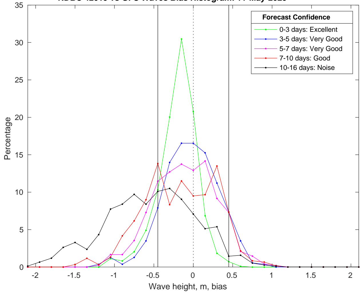
NDBC 42019 vs GFS Waves Bias Histogram: 11-May-2025
