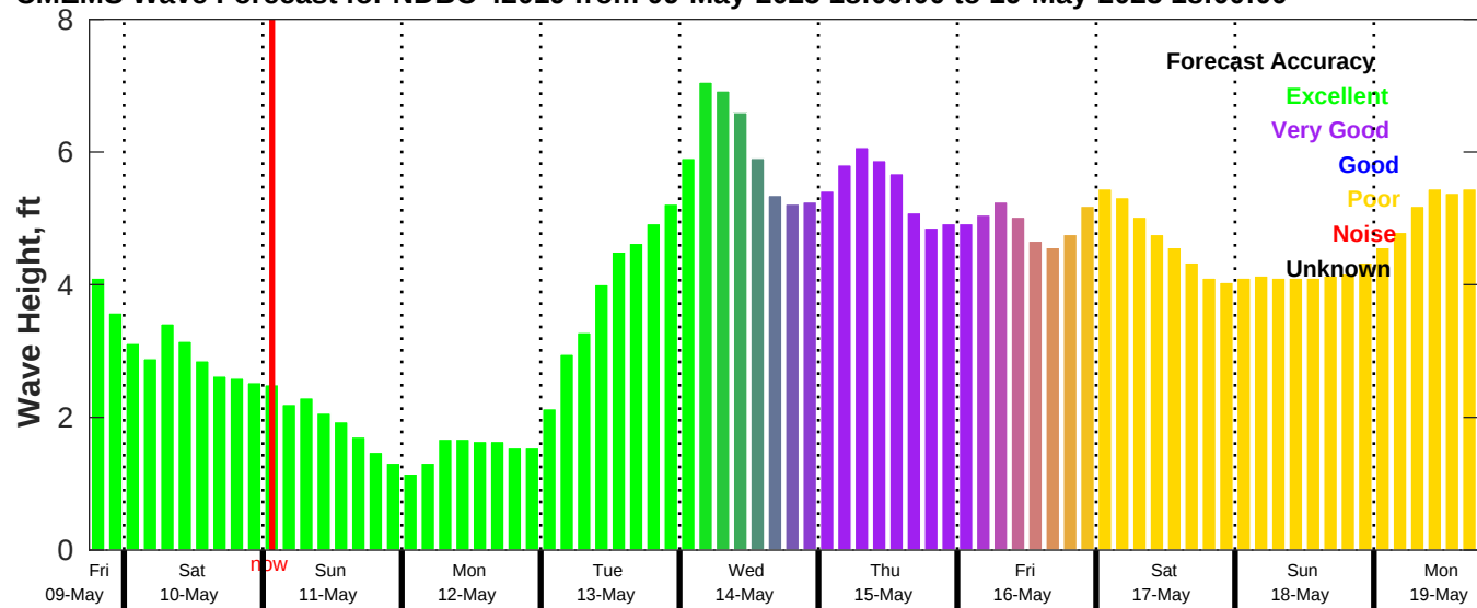
CMEMS Wave Forecast for NDBC 42019 from 09-May-2025 18:00:00 to 19-May-2025 18:00:00
