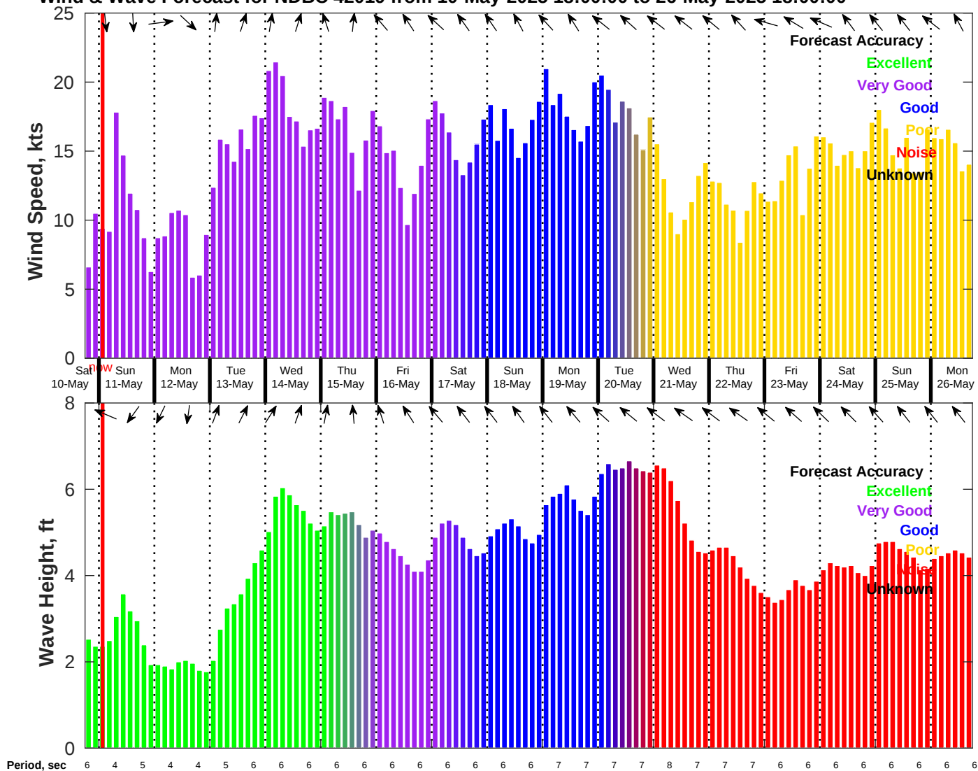
Wind & Wave Forecast for NDBC 42019 from 10-May-2025 18:00:00 to 26-May-2025 18:00:00
