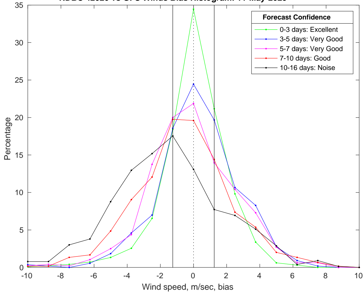
NDBC 42020 vs GFS Winds Bias Histogram: 11-May-2025
